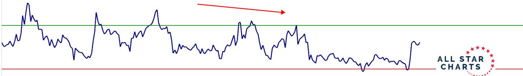
14 Period RSI
